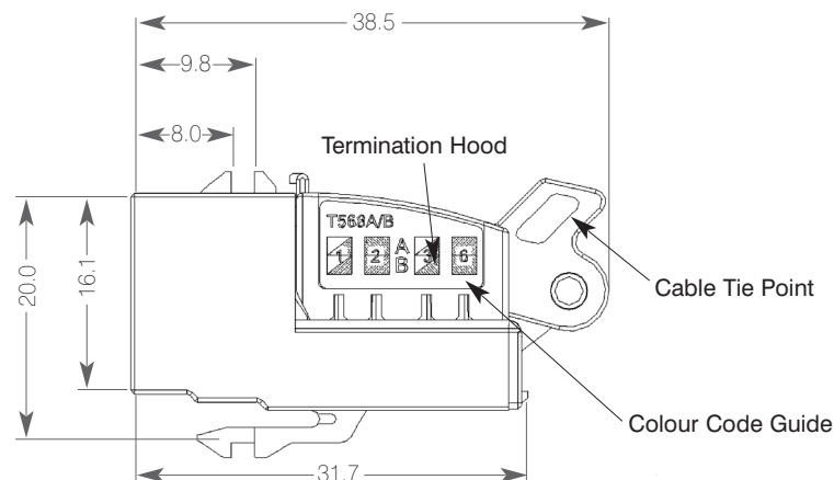
Side profile. All dimensions are shown in mm
