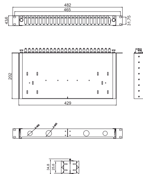
D. Product dimensions, front, plan and rear view and fixing arms, shown in mm
