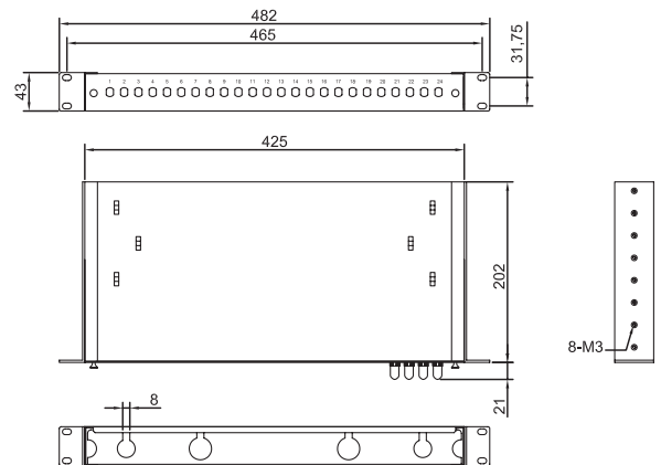
D. Product dimensions, front, plan and rear view and fixing arms, shown in mm
