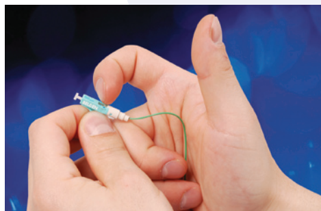
2. Using your index finger, slide the connector's switch-like activator tab toward the fibre to be terminated to bring about the splice/crimp
